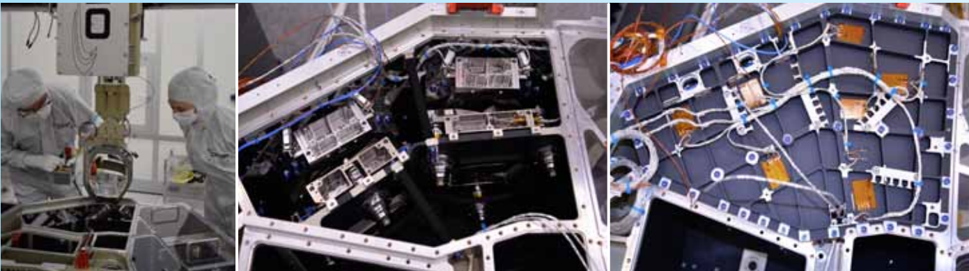
Instrument Optical Unit structure integrated with the pre-assembled Mirrors and Prisms, forming the EnMAP Spectrometer
